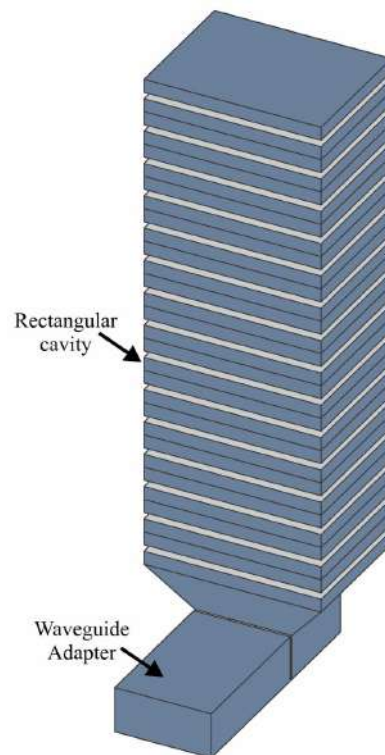
FIGURE 5.2: Rectangular resonating cavity charging setup with waveguide adapter and iris.
