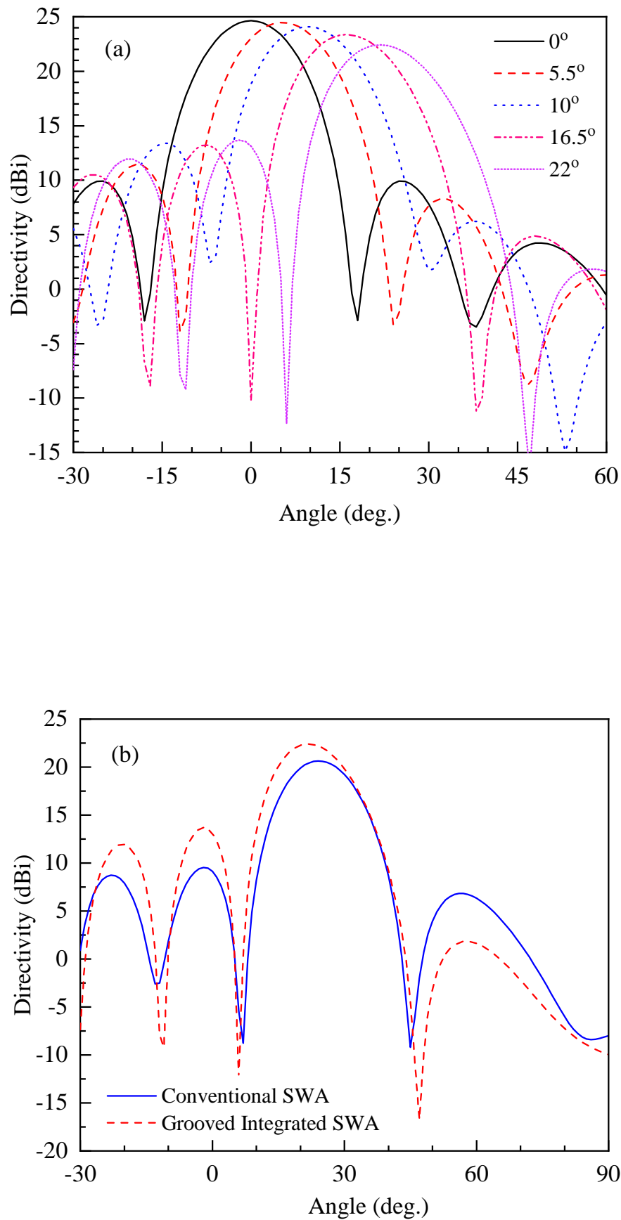
FIGURE 7.11: (a) Beam steering capability of a four element slotted waveguide array antenna (SWAA) system and (b) conventional (without grooved) vs proposed (with grooved) slotted waveguide array antenna (SWAA)
