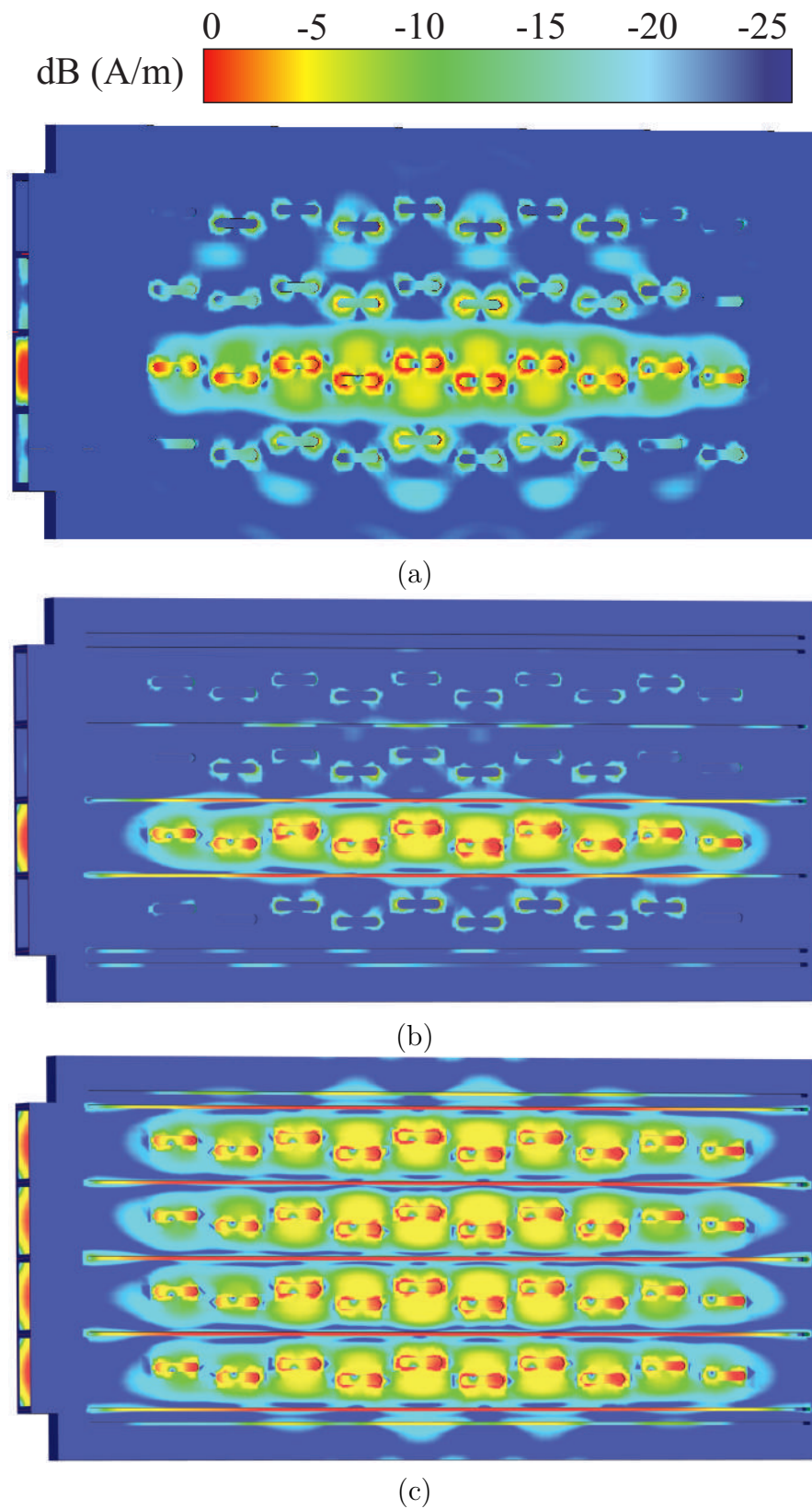
FIGURE 7.9: Surface current distribution pattern, in a four elements slotted waveguide array antenna, when only 3 rd element of the array is excited (a) without (b) with groove structure and (c) when all elements are excited
